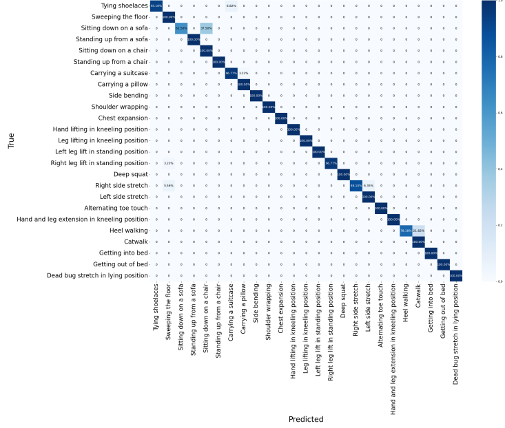
Fig. 3. The confusion matrix for the action classification result of our action recognition module.
