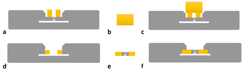
Fig. 2 Short sensor (a–c) and open sensor (d–f) made using AZ-9654 UHF RFID tags (grey) and conductive tapes (yellow)
